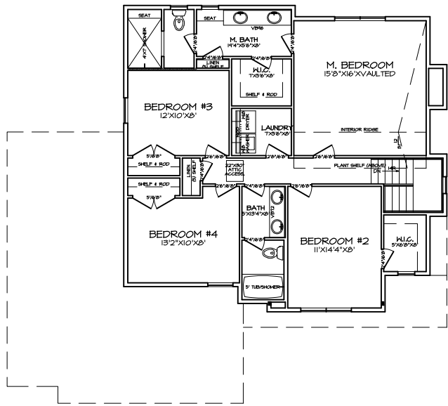
2 SECOND FLOOR PLAN A-4
